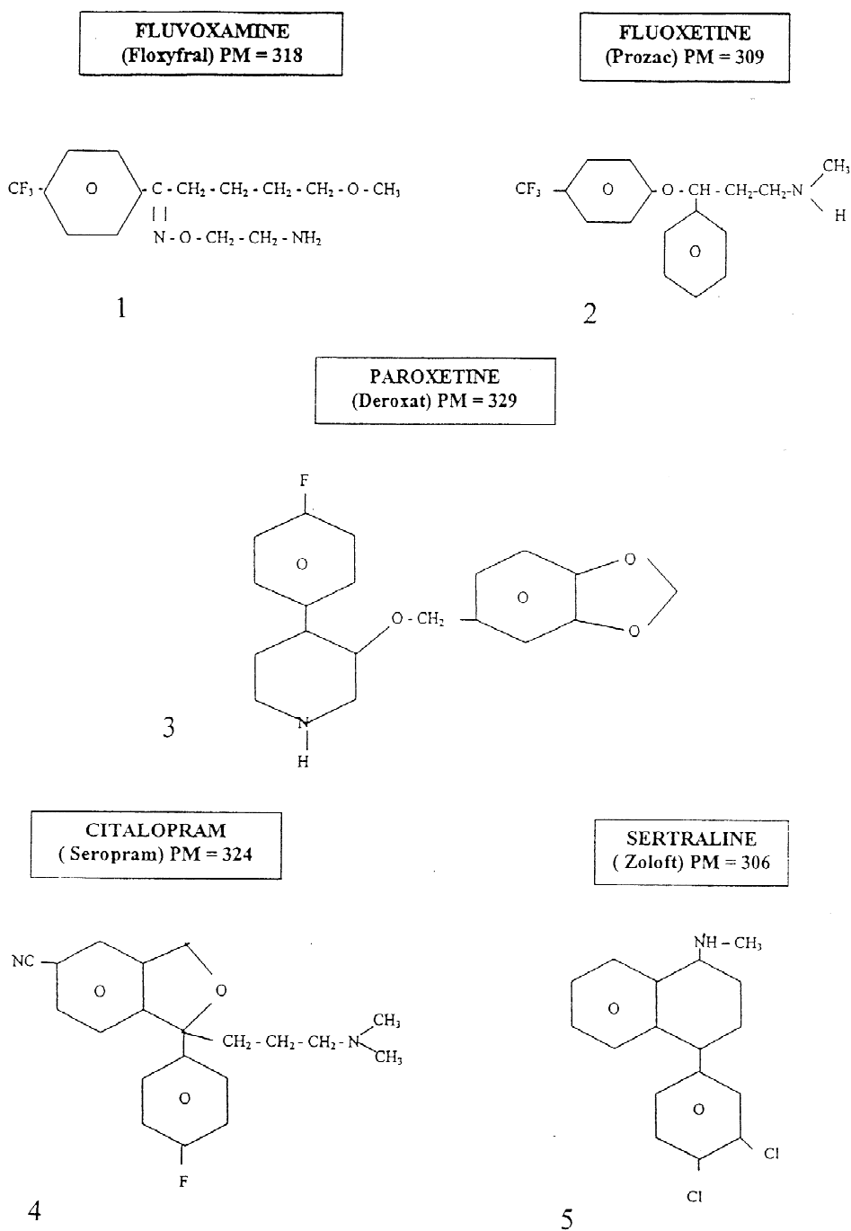
Fig. 1. Structure of selective serotonin reuptake inhibitors.
